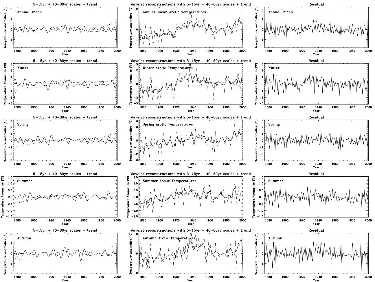
Figure 3. Reconstructed Arctic SAT anomalies accounting for variations on the decadal (5–15 years; solid lines), multidecadal (40–80 years; dashed lines) and the trend (dotted lines) scales by inverse wavelet transform. The results are shown individually in column 1, as the reconstructed sum (solid lines and original raw temperature records shown as dashed lines) in column 2, and as the residual between the 5–original raw series and the wavelet reconstructed series in column 3.
