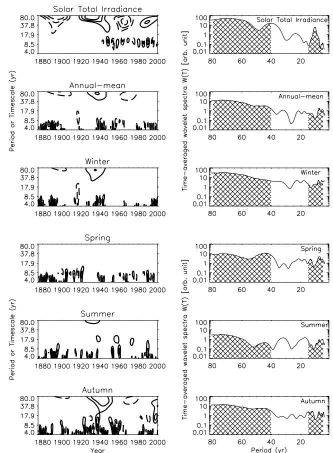
Figure 2. The time-frequency distribution of wavelet coefficients (left column) and the time-averaged wavelet spectra (right column) for all series. Negative contours/anomalies are dashed. Hatched areas under the time-averaged wavelet spectra are the broadband decadal (5–15 years) and multidecadal (40–80 years) forcing and response interaction scales assumed for the solar irradiance-Arctic SAT correlations studied here.
