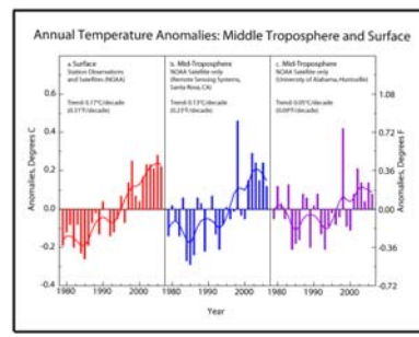
Surface -vs- Satellite Temps
